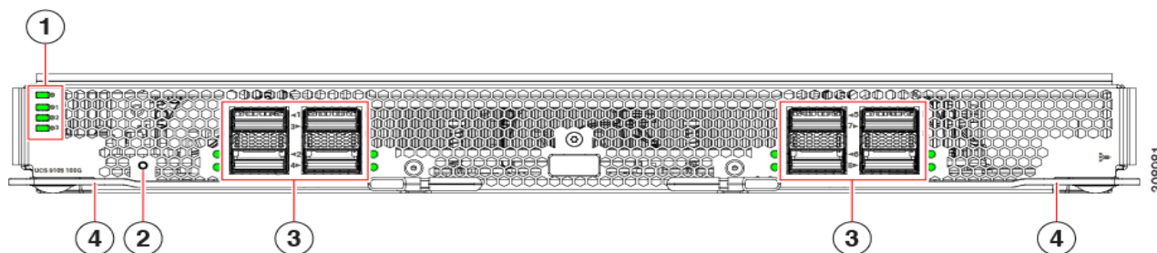
Figure 6 Cisco UCS 9108-100G IFM (front view)
