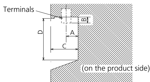
Terminal b 55SF2U Terminal (Bottom)
