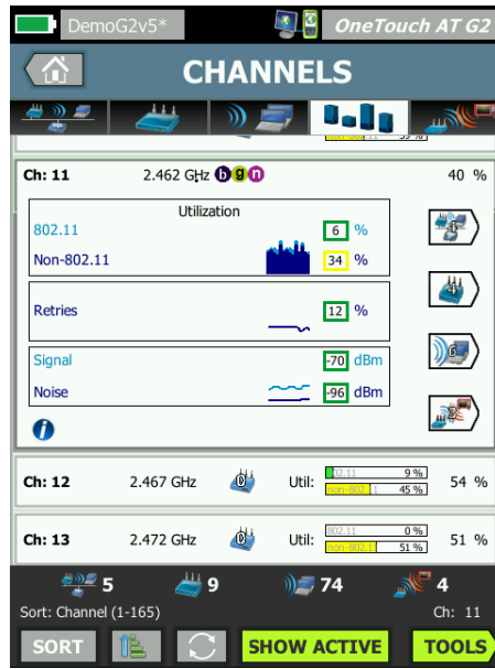
Figure 24: Visibility into each Wi-Fi channel, showing bandwidth occupied by 802.11 and non-802.11 traffic.
