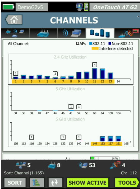
Figure 23: Analyze Wi-Fi health by each available channel.
