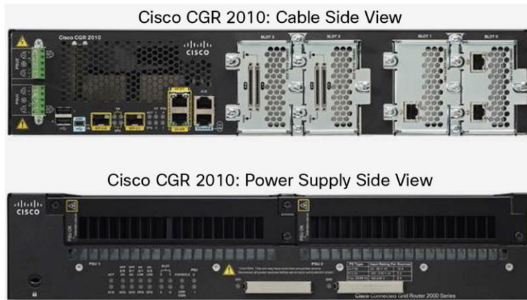
Figure 1. Cisco CGR 2010
