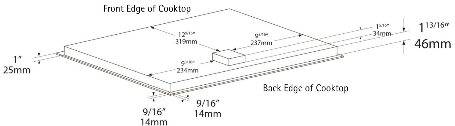
UNDERSIDE VIEW
