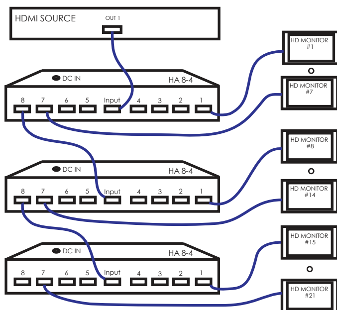
HDMI Distribution Amplifiers Cascade Configuration
