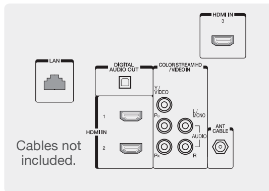
Rear Panel Connector Diagram
