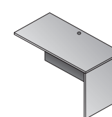
LOD45 Return Shell 48"x24"x29" CU:1.6 WT:57.2
