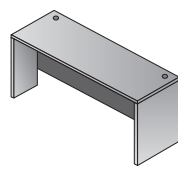
LOD03 Desk Shell 60"x30"x29" CU:3.0 WT:94.6
