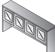
LOD41 Overhead with Wood/ Glass Doors 71"x14"x36" CU:4.7 WT:121 Consists of: NAP-44H,4DC
