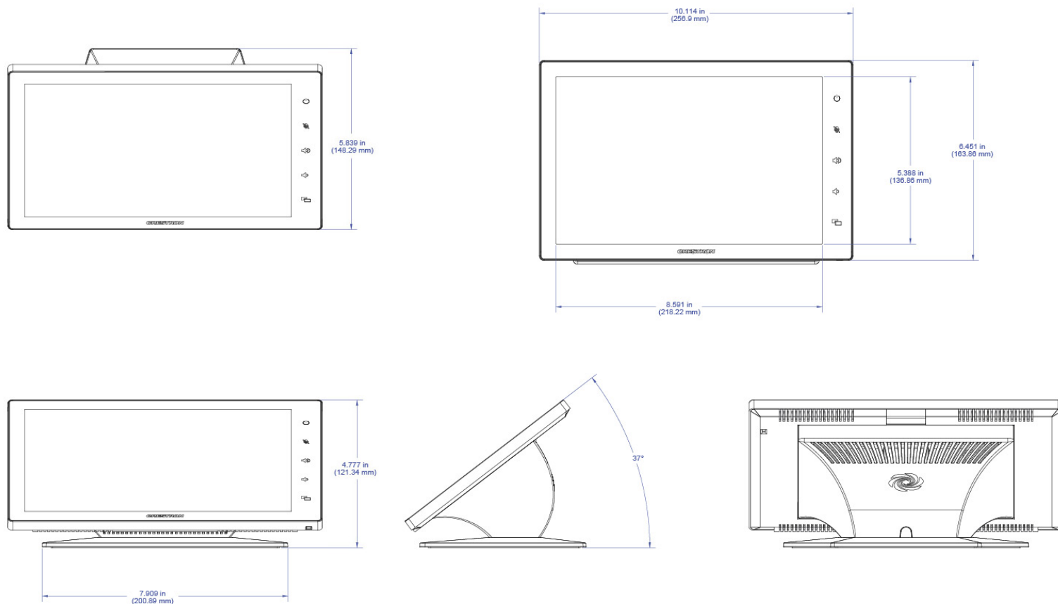
10" Tabletop Touch Screen
