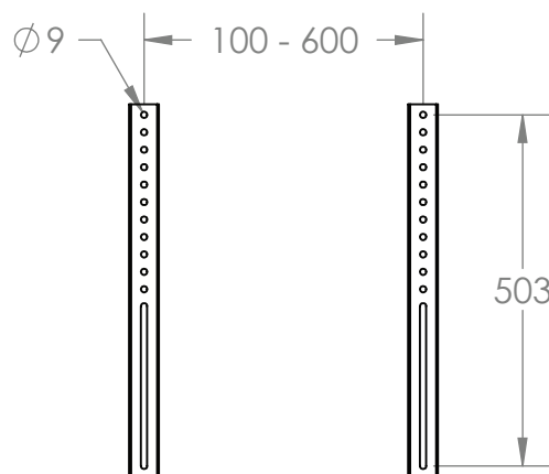
PANEL ATTACHMENT - VESA COMPATABILITY (mm)
