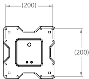
PANEL ATTACHMENT - VESA COMPATABILITY (MM)
