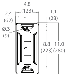
WALL MOUNTING
