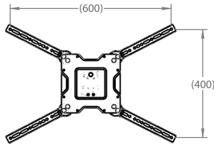
PANEL ATTACHMENT - VESA COMPATIBILITY (mm) WITH ADAPTERS
