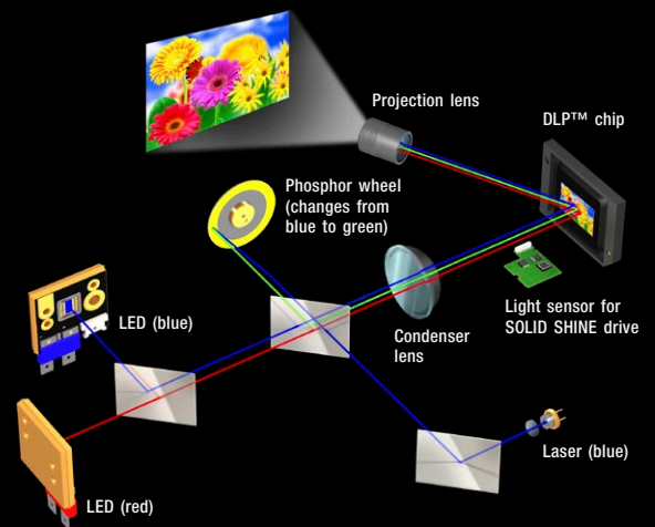
PT-RZ370/RW330 Optical Structure Image
