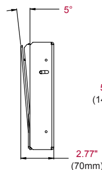
Side View Tilt
