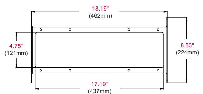
Adapter Detail
