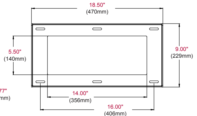
Wall Plate Detail
