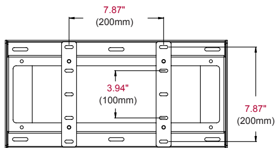
Front View VESA 200 x 200 VESA 200 x 100
