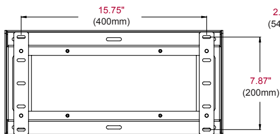
Front View VESA 400 x 200
