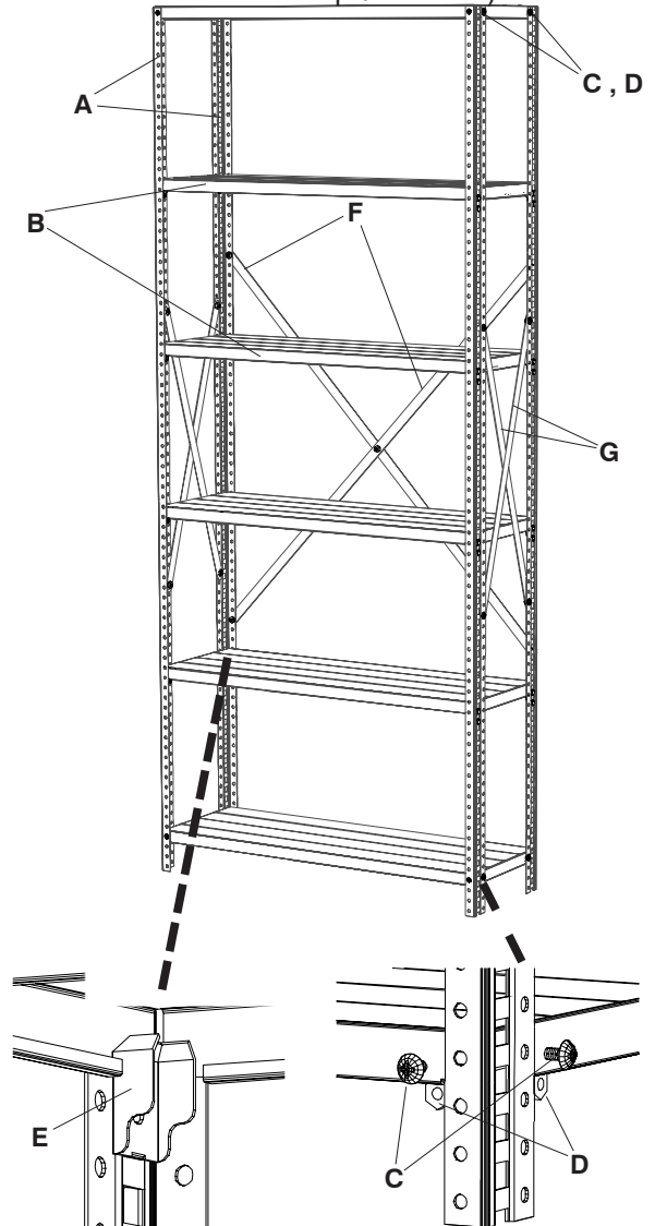
Assembled Unit (5256 Post Pack and 5250 Shelf pack shown)
