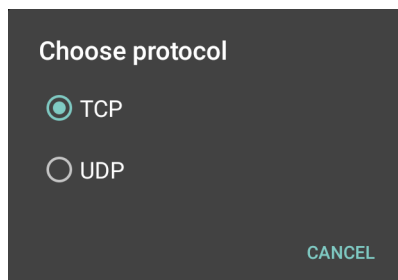
Figure 134 Protocol Selection
