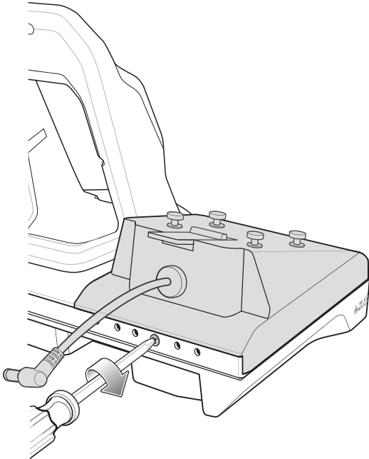
Figure 77 Secure adapter to Cradle
