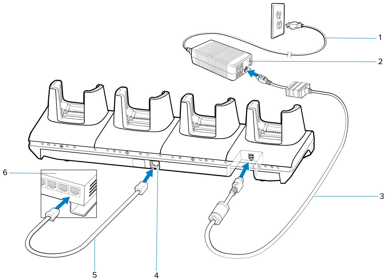
Figure 21 4-Slot Ethernet ShareCradle Setup
