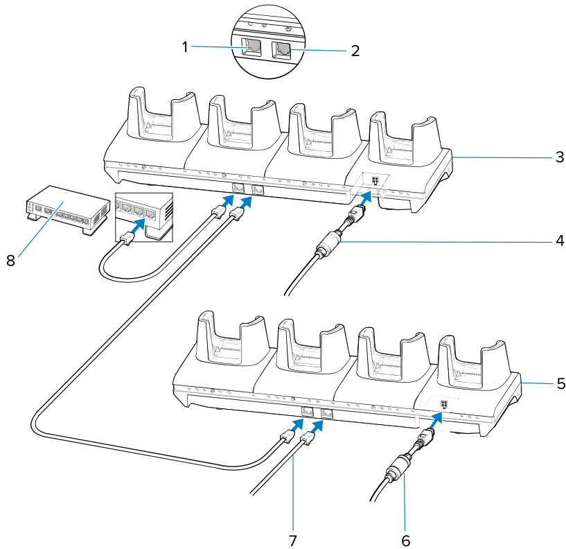
Figure 23 Daisy-chaining 4-Slot Ethernet ShareCradles
