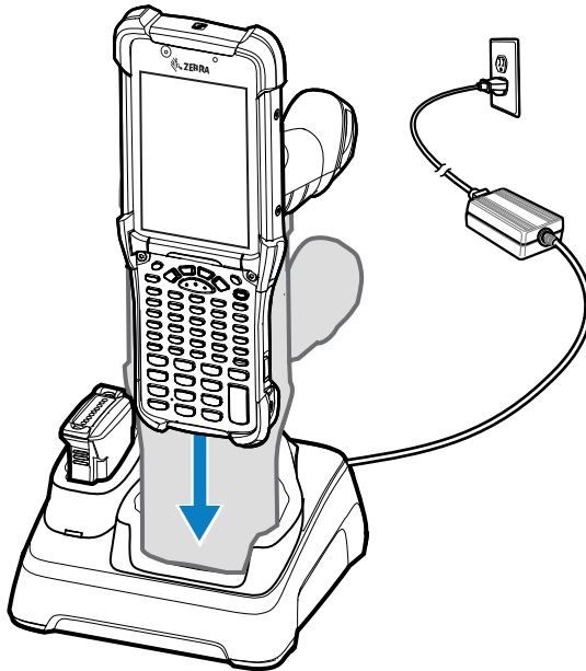
Figure 16 1-Slot USB Charge Cradle with Spare Battery Charger
