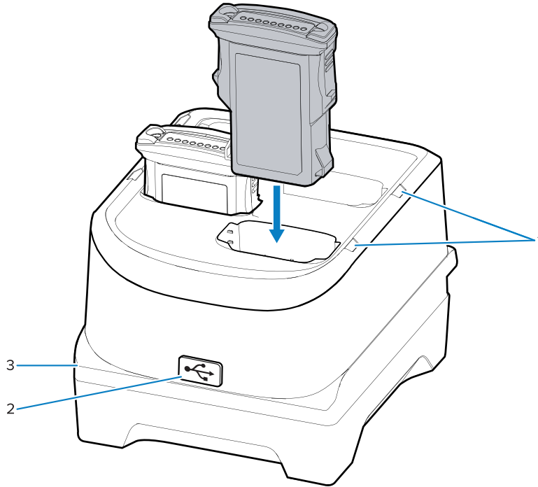
Figure 26 4-Slot Spare Battery Charger
