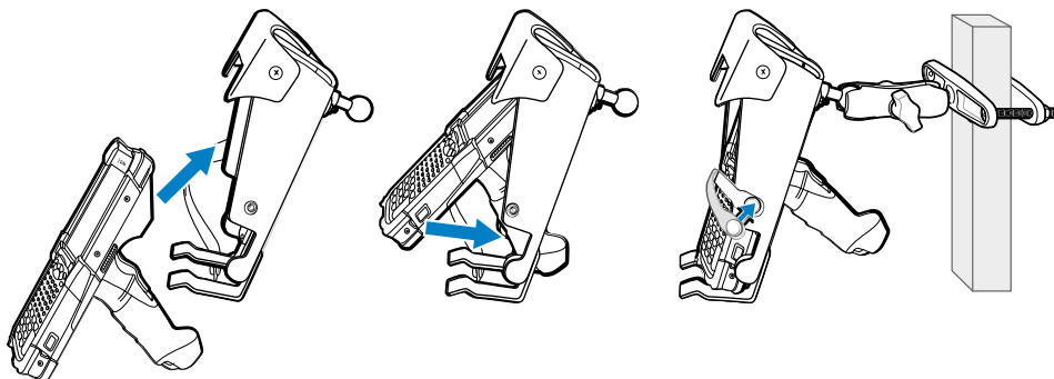
Figure 37 Insert Device into Forklift Mount Holder, Rotate and Snap (Option 2)
