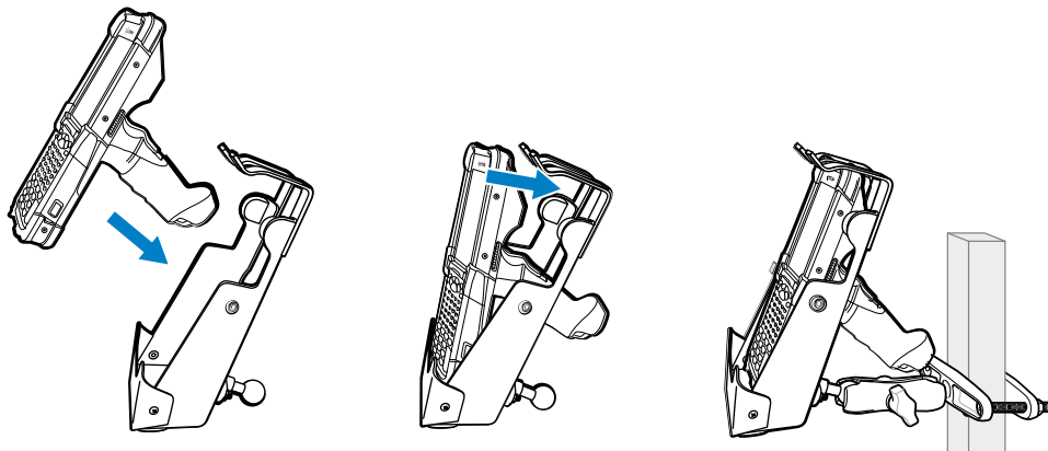
Figure 37 Insert Device into Forklift Mount Holder, Rotate and Snap (Option 2)
