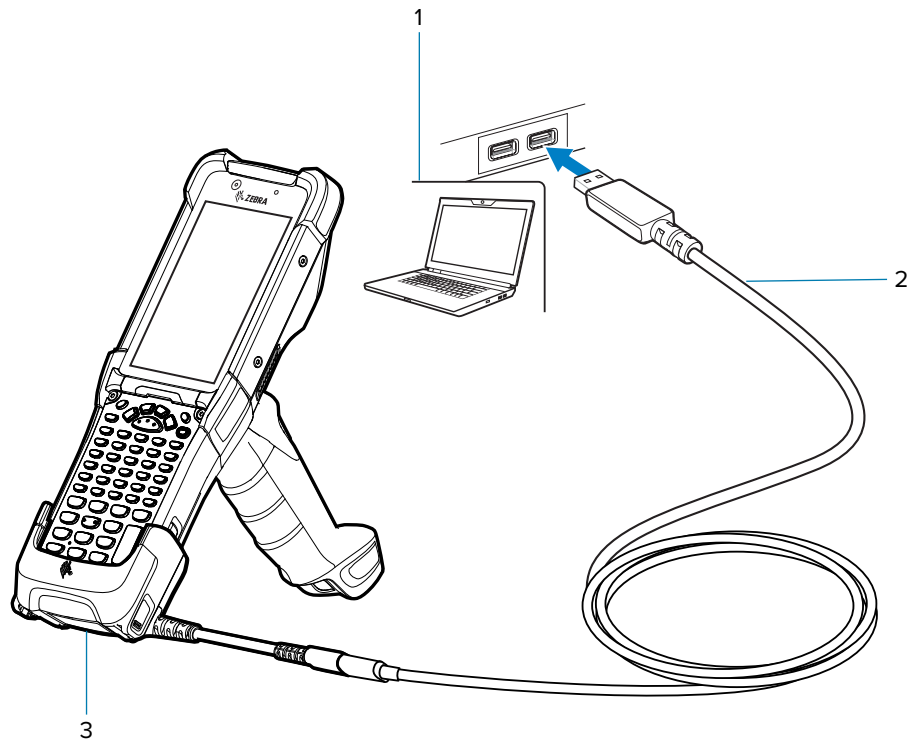
Figure 32 Connecting USB Charge/Com Snap-on Cup to Host Computer
