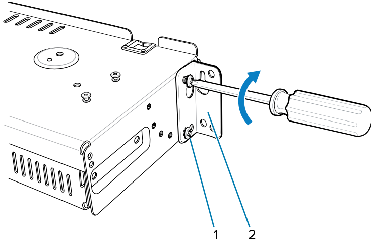
Figure 38 Flange Horizontal Position (5-Slot Cradles)
