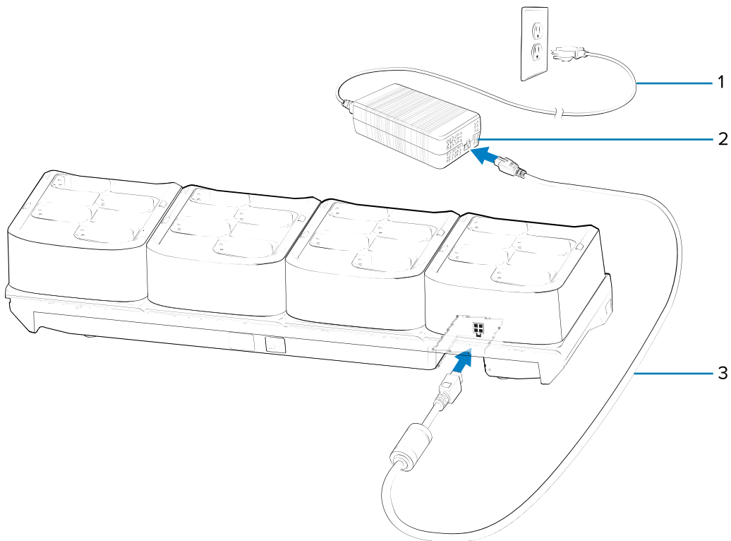
Figure 28 16-Slot Spare Battery Charger Setup
