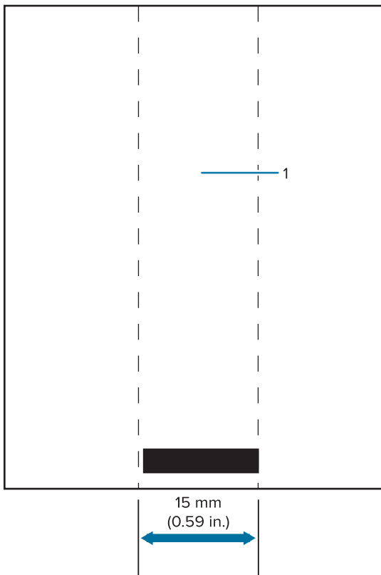
Figure 26 Label Areas
