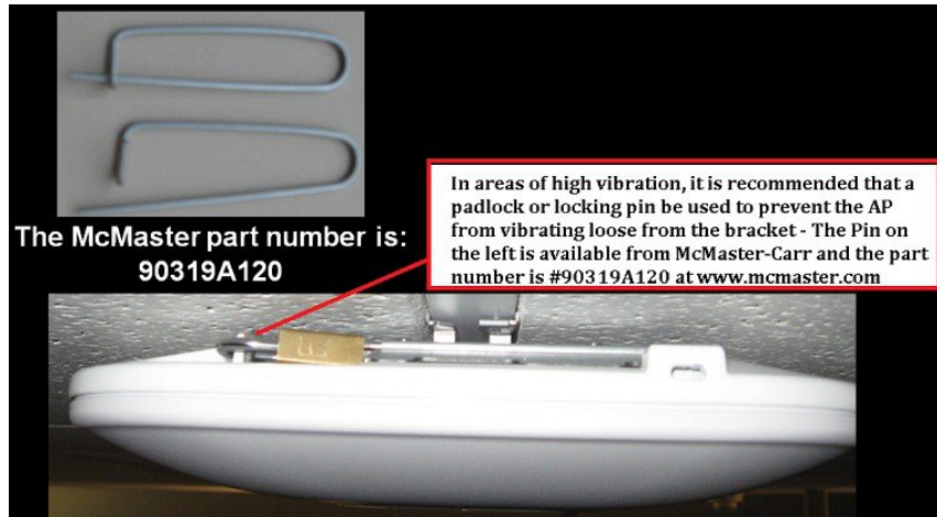
Figure 56: Metallic Parts
