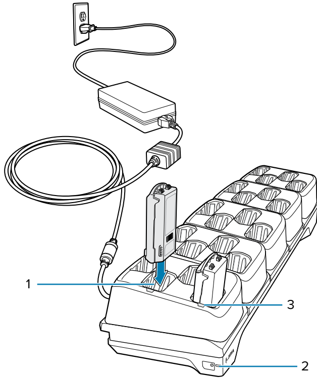
Figure 40 20-Slot Spare Battery Charger
