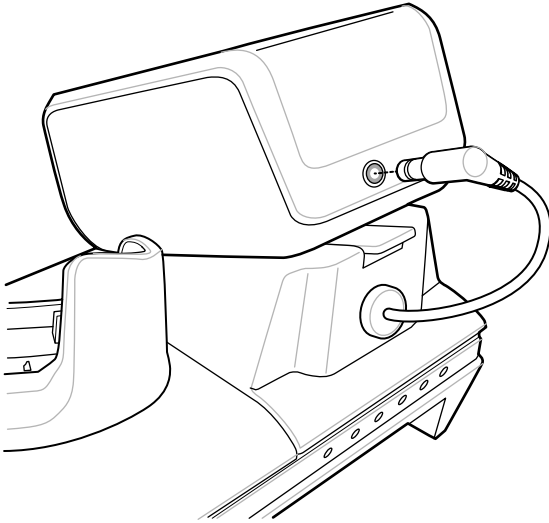
Figure 42 Connect Charge Only Cradle Power
