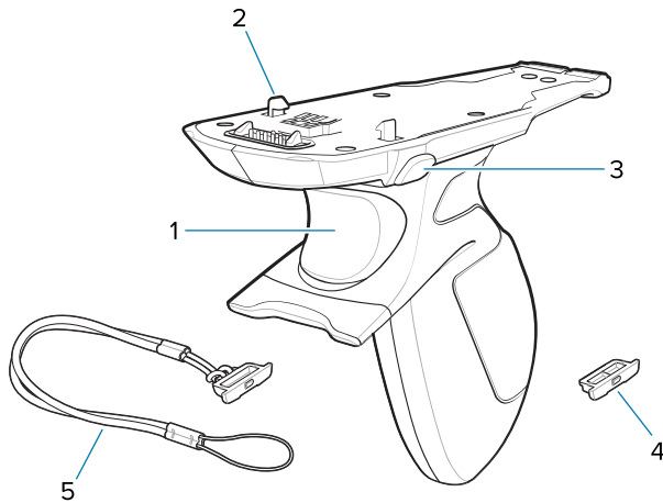
Figure 49 Trigger Handle
