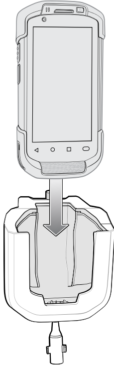
Figure 51 Install Device into Vehicle Cradle
