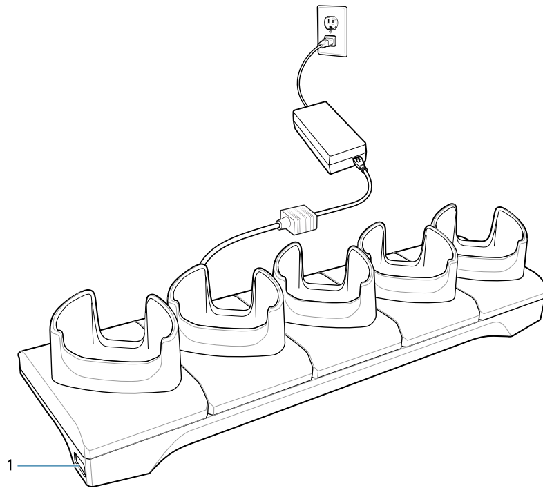
Figure 38 5-Slot Charge Only Cradle
