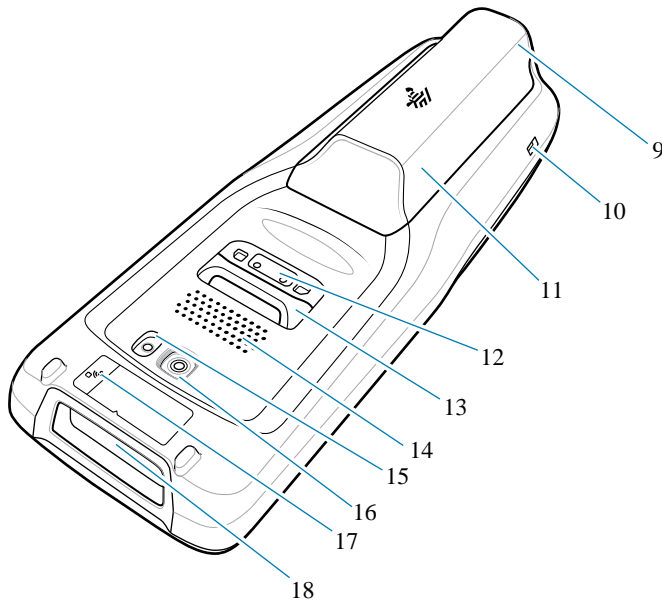
Figure 2 Back View
