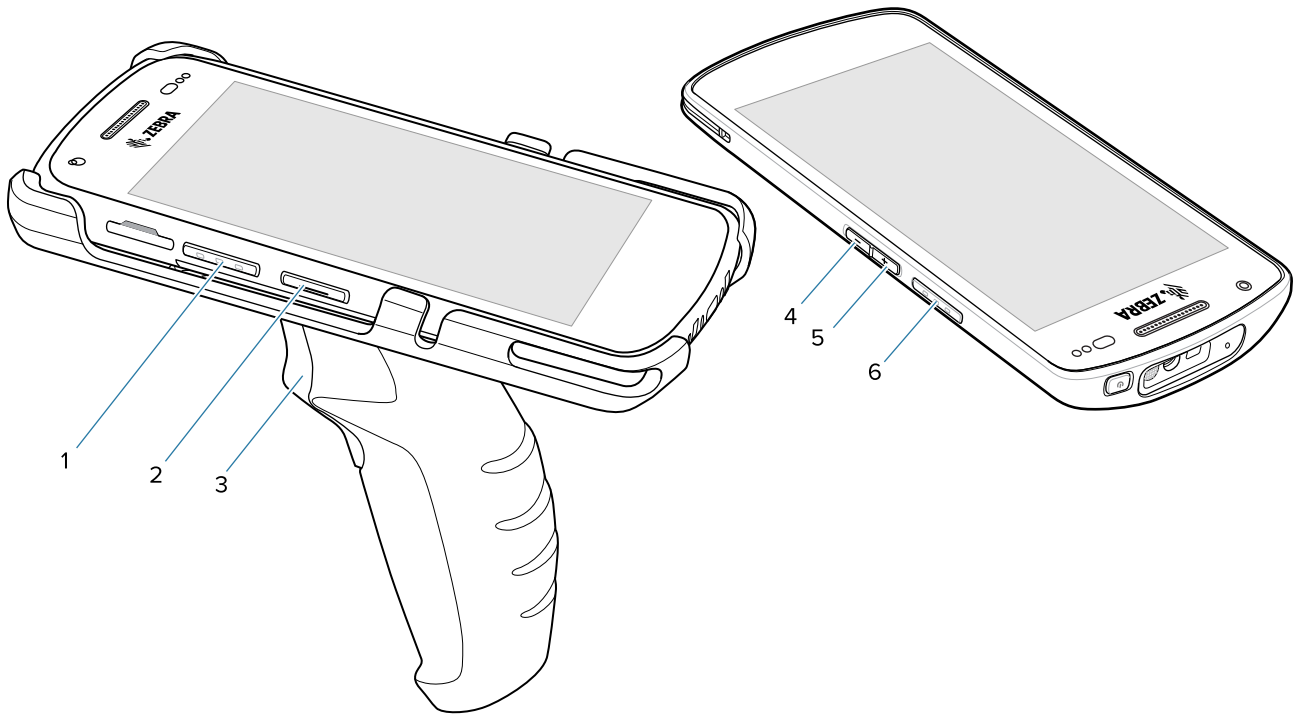
Figure 6 Key Positions
