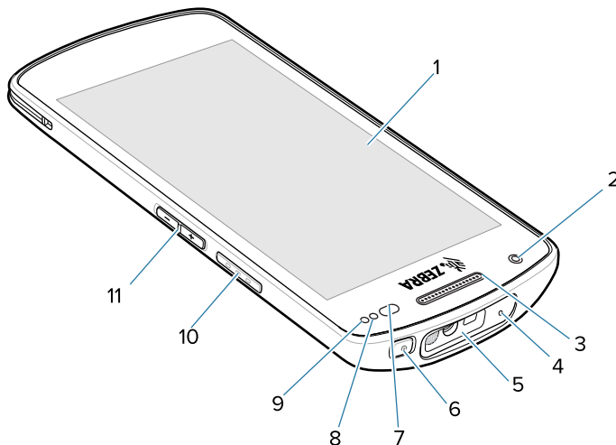
Figure 1 Front View
