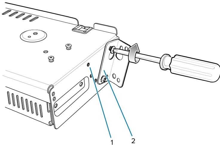
Figure 41 Flange 25° Position (4-Slot Battery Chargers)
