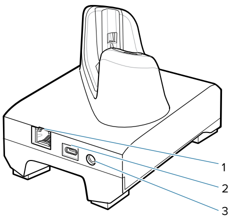
Figure 25 Back View
