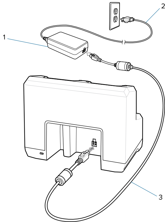
Figure 30 4-Slot Locking Charge Only Cradle
