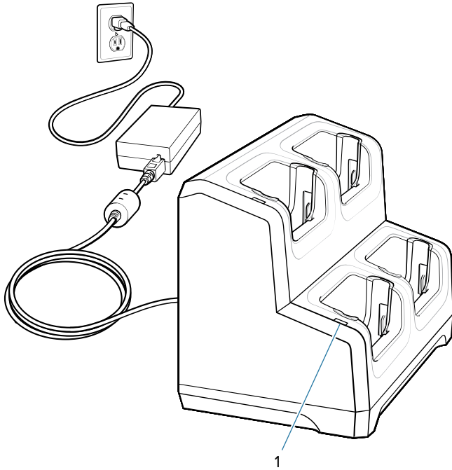
Figure 29 4-Slot Charge Only Locking Cradle Features
