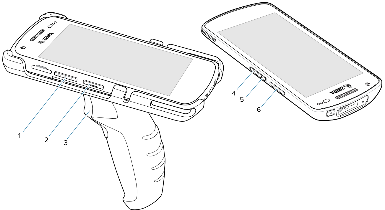
Figure 6 Key Positions
