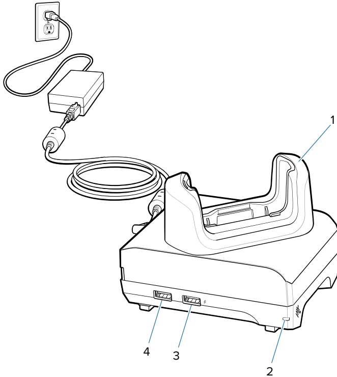
Figure 32 Front Left View
