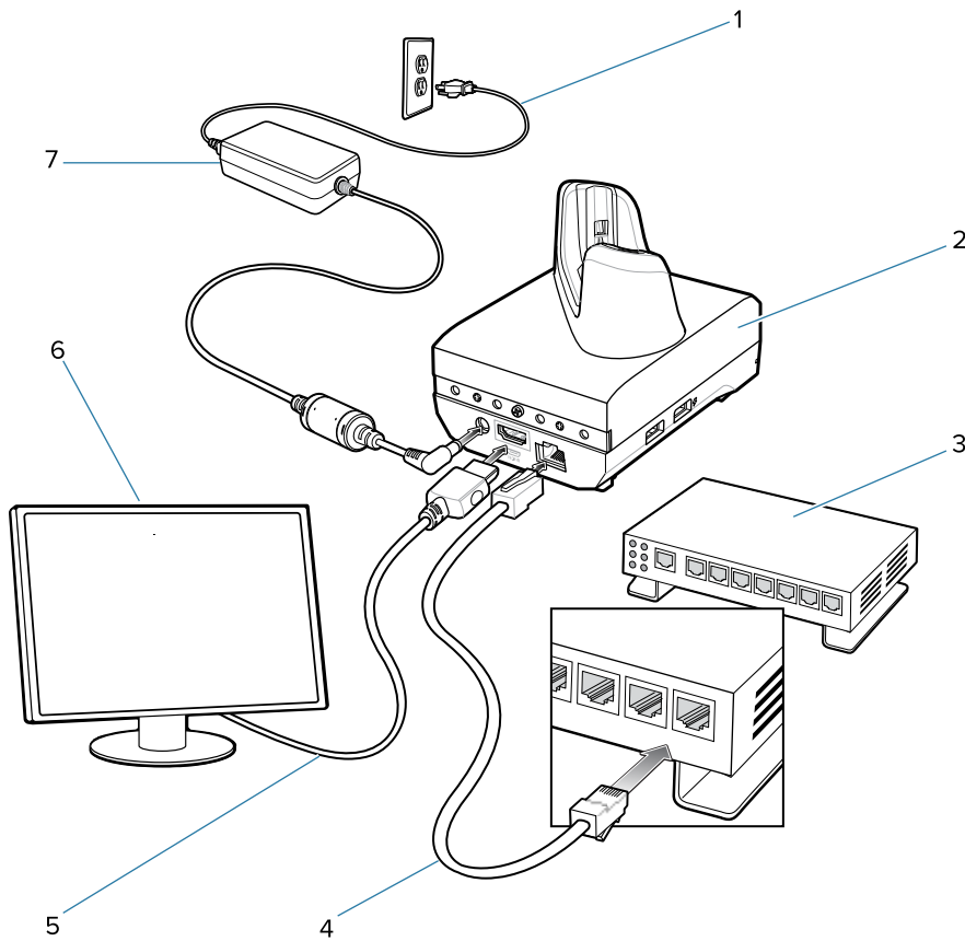
Figure 34 Workstation Cradle Setup
