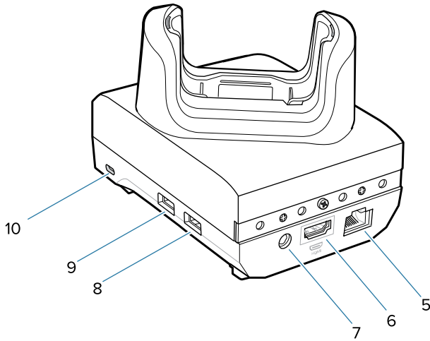
Figure 33 Rear Right View
