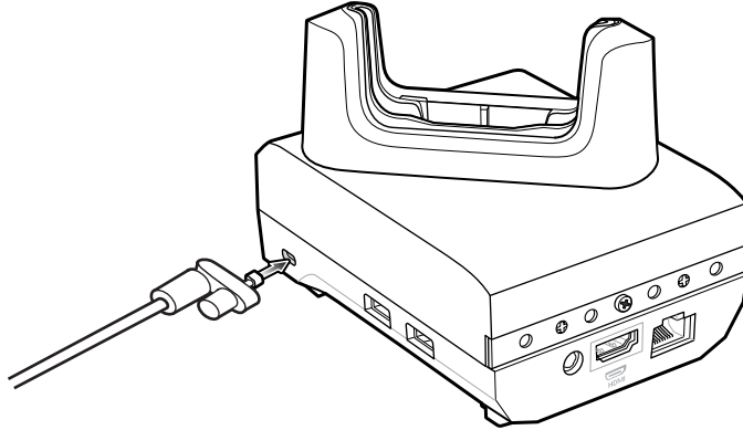
Figure 35 Securing Cradle with Kensington Lock
