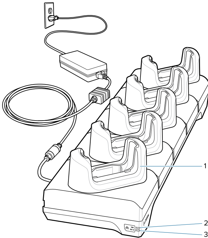
Figure 37 5-Slot Ethernet Cradle
