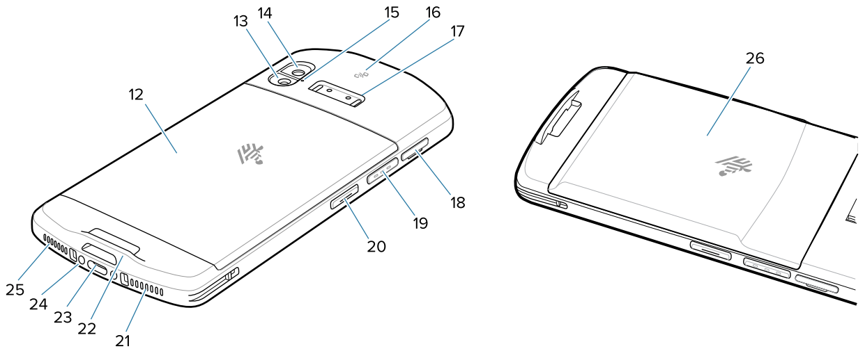
Figure 2 Rear View
